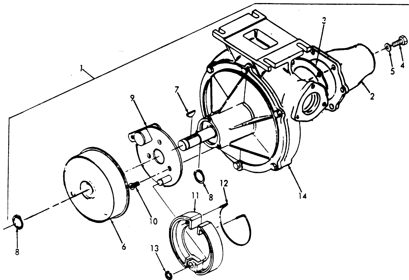
Figure No. 13 Pump And Brake
