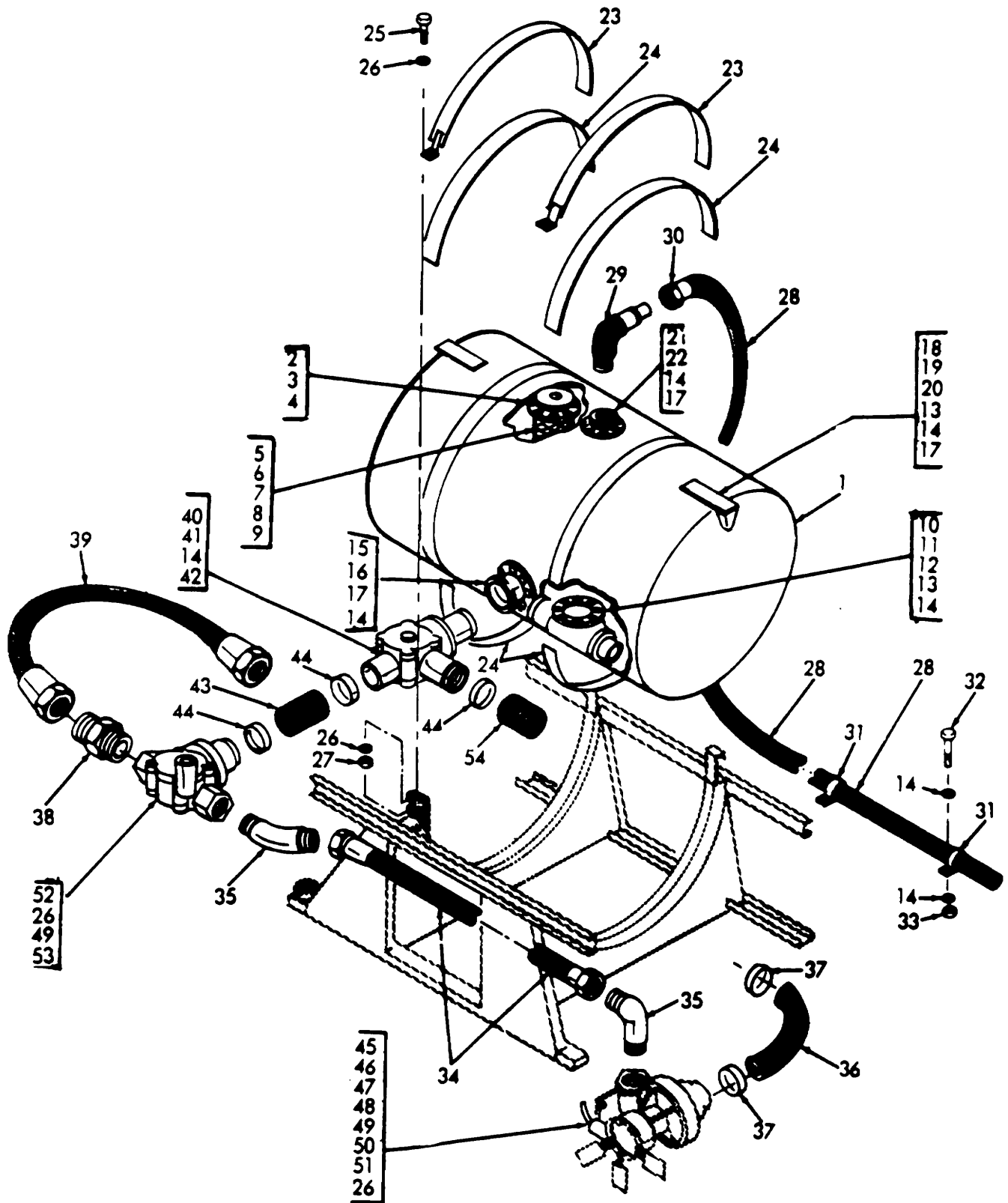
Figure No. 8 Spray Tank And Related Parts 28
